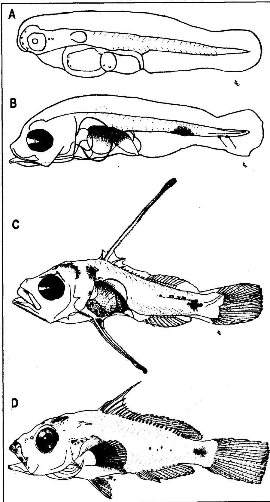
Figure 3. Developmental stages of laboratory-reared Nassau grouper (from Powell and Tucker, 1992, with permission from the Bulletin of Marine Science):
