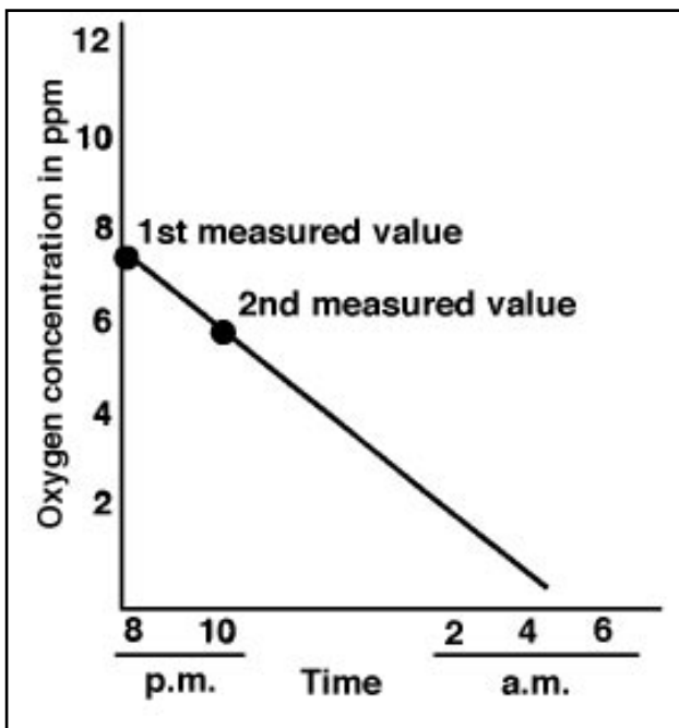
Figure 1. Graphic method of predicting nighttime oxygen depletions in ponds. In this example it is predicted the oxygen concentration will drop to 2 ppm by 2:40 a.m., indicating emergency aeration should be started by 3:30 a.m.
